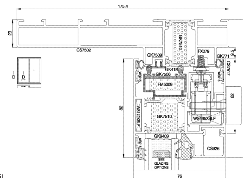
Double Track Security Interlock Option for Secured by Design, PAS24:2016
