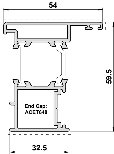
ETC648 Meeting Stile For French Casement
