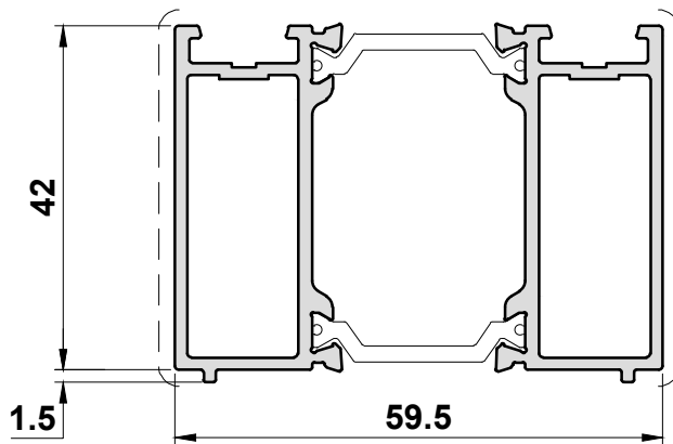
ETC652 42mm Frame Extension
