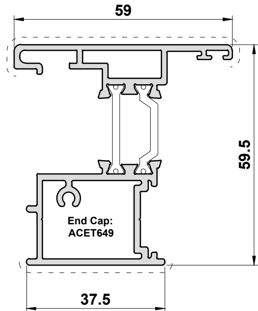
ETC649 Meeting Stile For French Casement
